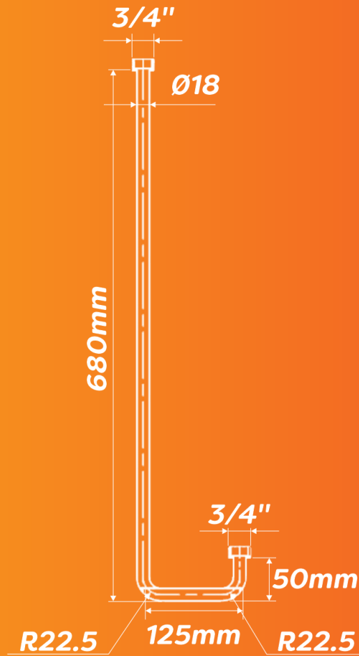
Top Entry Pipe
